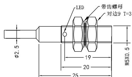
HIM05E-0B8NO-S1/01BNO-S1/1B2NO-S1
