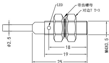
HIM04E-0B6NO-S1/0B8NO-S1/01BNO-S1
